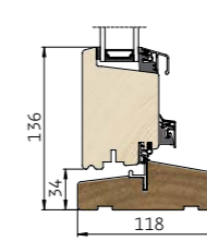
2 Lodret snit i bundkarm/ramme
