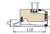
2 Lodret snit i bundkarm/ramme
