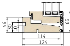
2 Lodret snit i bundkarm/ramme
