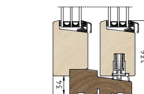
2 Lodret snit i bundkarm/rammer
