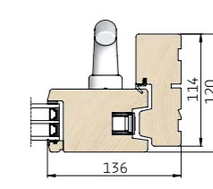
2 Lodret snit i bundkarm/rammer
