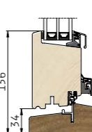
2 Lodret snit i bundkarm/ramme
