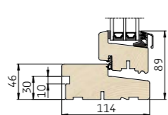
2 Lodret snit i bundkarm/ramme
