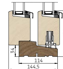
2 Lodret snit i bundkarm/rammer
