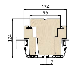
4 Vandret snit i midtkarm/rammer
