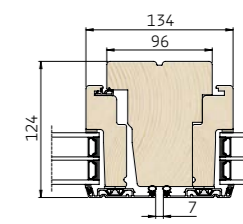
4 Vandret snit i midtkarm/rammer
