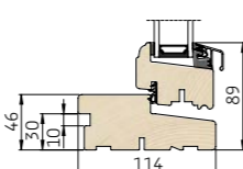
3 Lodret snit i bundkarm/ramme
