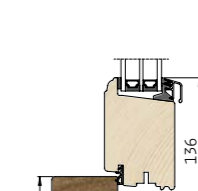
3 Lodret snit i bundkarm/ramme
