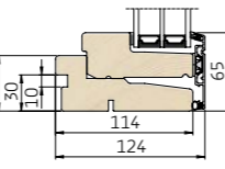
3 Lodret snit i bundkarm/ramme
