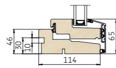
2 Lodret snit i bundkarm/ramme
