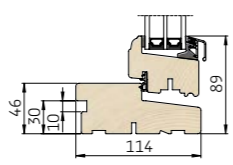
3 Lodret snit i bundkarm/ramme
