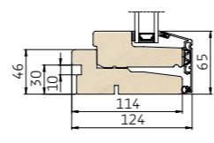
3 Lodret snit i bundkarm/ramme
