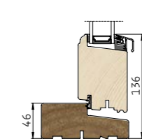
3 Lodret snit i bundkarm/ramme
